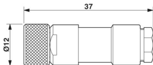
Socket M8 x 1, straight
